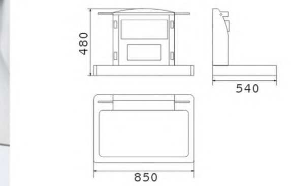
11W004 婴儿护理台 Baby nursing surface
